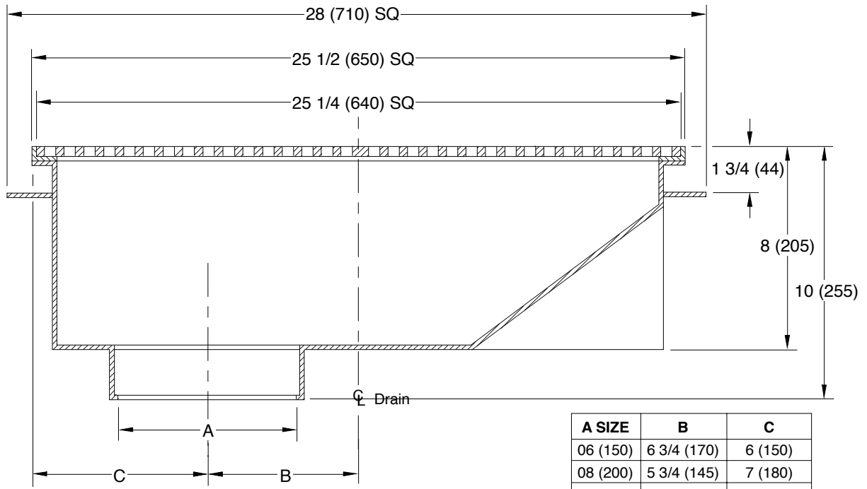
Fig. 6060C . . . CAULK OUTLET ONLY
