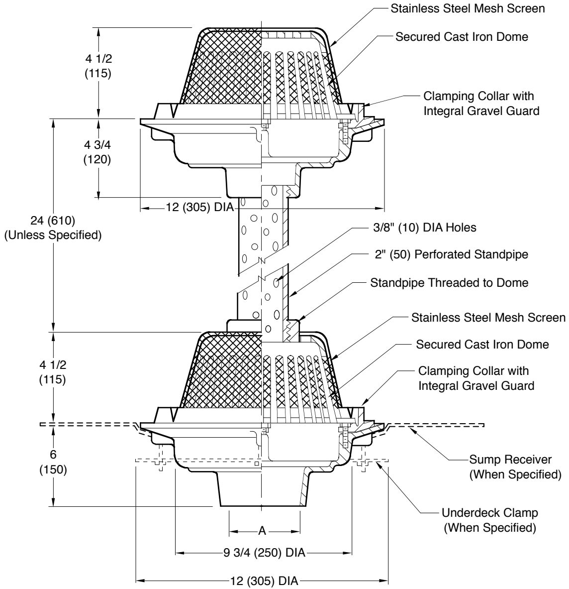
Fig. 1915 . . . NO-HUB Outlet
