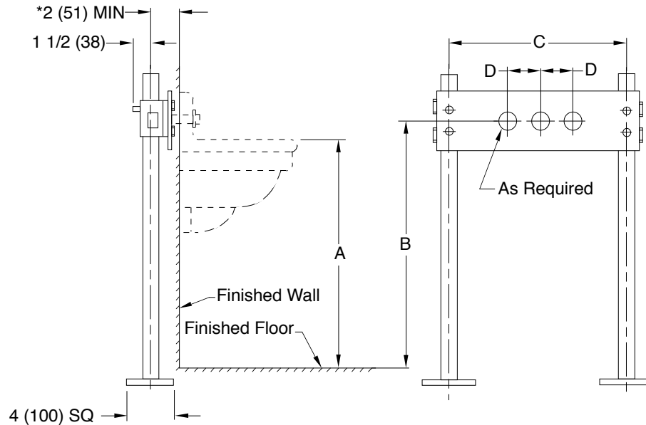
Fig. 0844 . . . FOR HIGH BACK INSTITUTIONAL TYPE LAVATORIES
