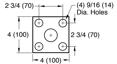
BASE DETAIL
