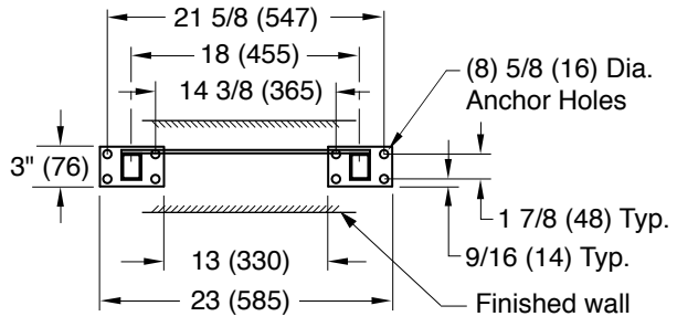
BASE DETAIL
