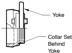
DETAIL OF COLLAR AND YOKE ASSEMBLY Fig. 0630
